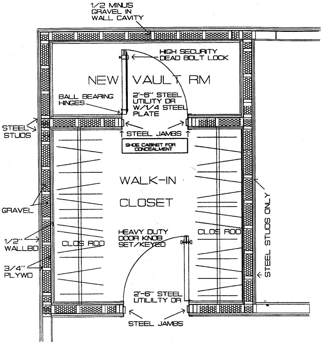
CLOSET FRAMING
